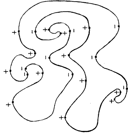
FIGURE 1. C(t) with critical points labelled.
